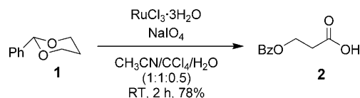
Scheme 1. Direct oxidation of the benzyldene acetal 1 to the \beta -benzoyloxy carboxylic acid 2 . Bz = benzoyl.
